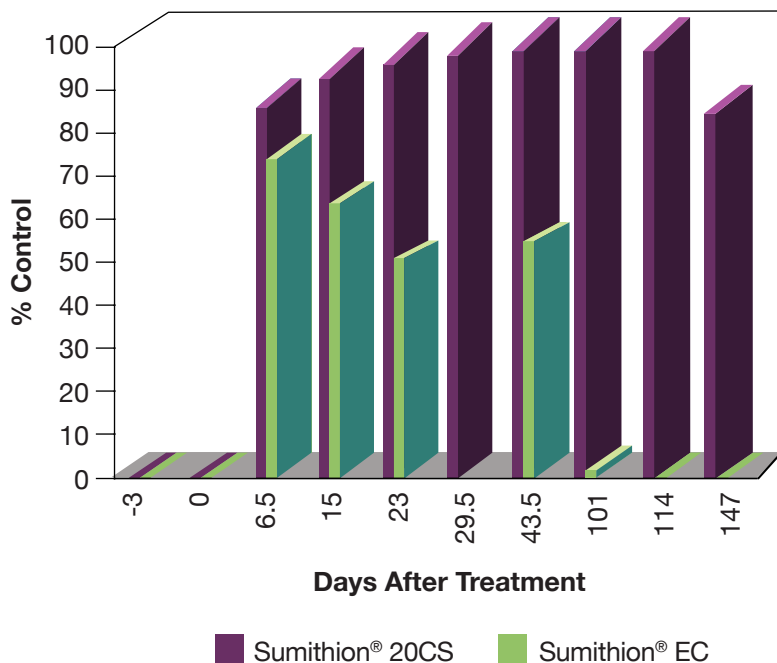
Activity of Sumithion® 20CS against cockroaches ( Blatella germanica ) in a field trial comparison with Sumithion® EC
